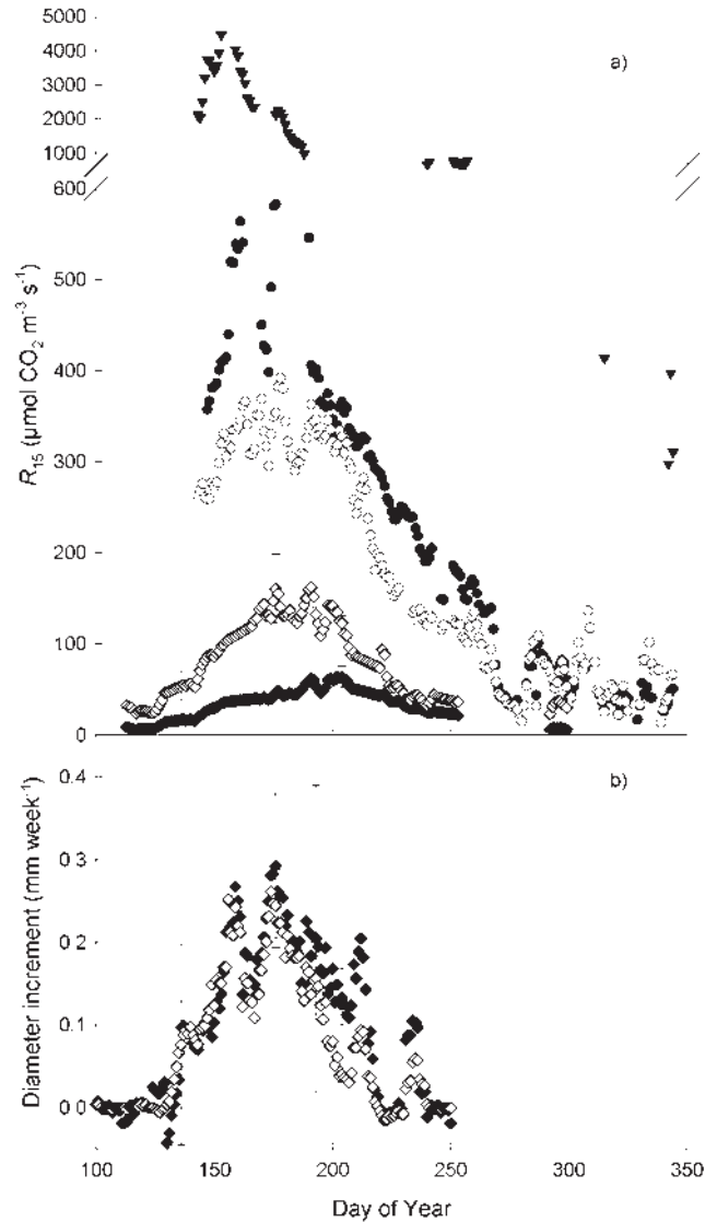
Figure 1. Seasonal and spatial variation in (a) stem respiration normalised to 15 °C ( R_{15} ) and calculated on a volume basis at breast height ( \blacklozenge , three to four cuvettes per point) and in the middle of the stem ( \diamond , three cuvettes per point) in 1998 and at the base ( \bullet ), middle ( \circ ) and top ( \blacktriangledown ) of the crown in 1997 of dominant 25-year-old beech trees at Hesse; (b) averaged stem diameter increment at breast height ( \blacklozenge ) and in the middle of the stem ( \diamond ) in 1998. The error bars represent the standard errors of the mean for the 1998 measurements and are presented for each of the four dates for which the standard errors were maximum for either the respiration rates or the diameter increments at breast height or in the middle of the stem. For further details, see text.
