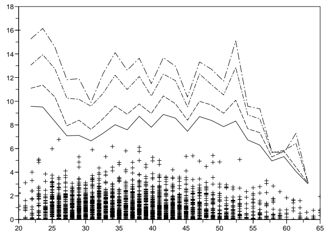
Figure 5: AIDS data: estimation of the conditional extreme quantile of the survival time. Full line: level \varepsilon = 0.01 , dashed line: level \varepsilon = 0.005 , dashed-dotted line: \varepsilon = 0.002 , dotted line: level \varepsilon = 0.001 . x -axis: age of the patient at the time of diagnosis, y -axis: survival time (in years).
