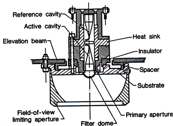
Schematic diagram of SERB-SR radiometer
