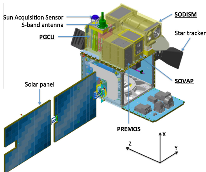
Fig. 9 MYRIADE platform example with the PICARD microsatellite.
