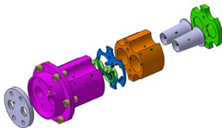
SERB-OS Optical sensor
