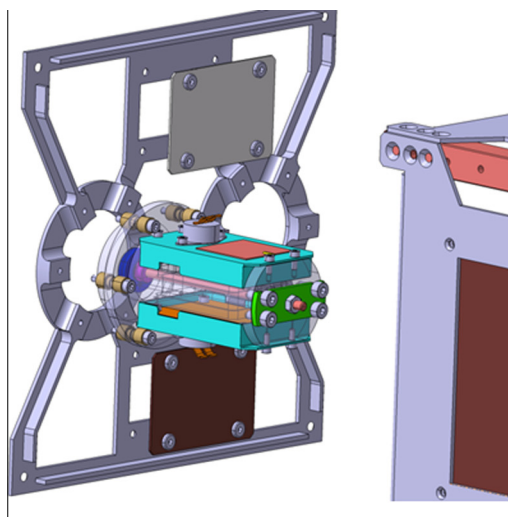
SERB-B Bolometer
