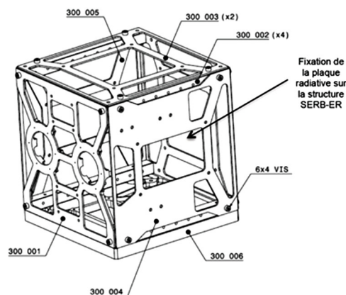
SERB-ER Radiometer (radiative plate)
