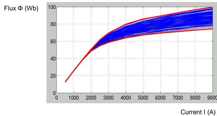
Fig. 13. 200 realizations of the flux \Phi in function of the excitation current I
