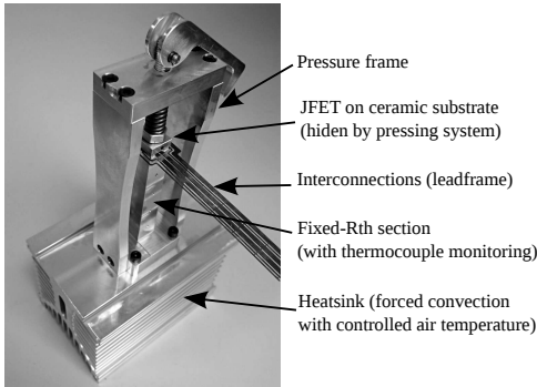
Fig. 6. The test support, showing the pressing frame, the location of the test vehicle, and the heatsink. Thermal insulation (not shown) is used to ensure that all the heat dissipated by the die is evacuated through the heatsink.
