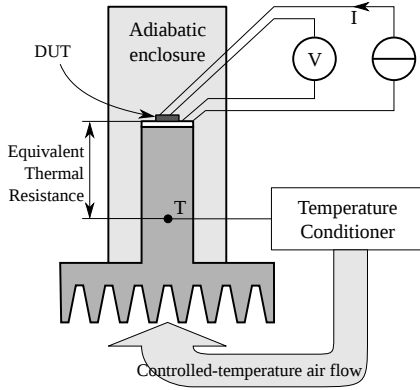
Fig. 5. Principle of the runaway test bench: the Device Under Test (DUT) is connected to a current source and the voltage across the DUT is measured. Its gate and source terminals are short-circuited to ensure it is “fully-on”. The thermal environment is controlled using a thermal conditioner to achieve a constant temperature at point T, regardless of the heat dissipated by the DUT.
