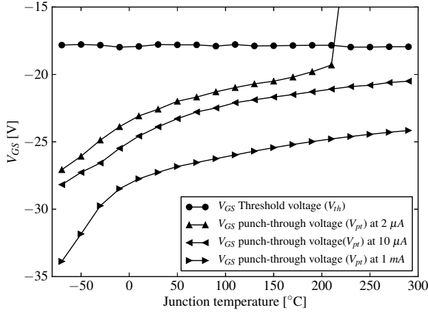
Fig. 3. Evolution of the gate-to-source punch-through voltage ( V_{pt} ) and the gate-to-source threshold voltage ( V_{T0} ) with temperature, for JFET #1. The punch-through voltage is measured at 2 \mu\text{A} , 10 \mu\text{A} and 1 \text{mA} gate current.
