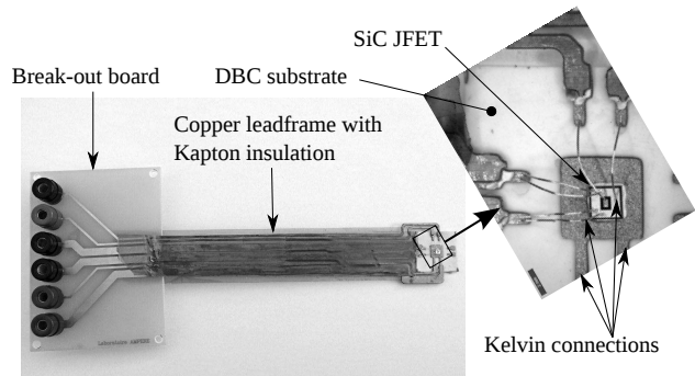
Fig. 2. Details of the high-temperature test vehicles
