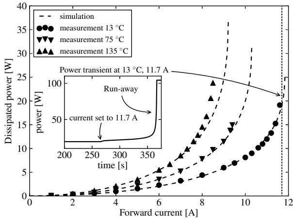
Fig. 8. Power dissipated by JFET #2 (7.9 K/W). The device entered (destructive) runaway at 11,7 A, 13 °C ambient temperature.
