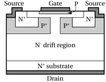
Fig. 1. Internal structure of the SiC JFET from SiCED [10]. This transistor is used in the present study.
