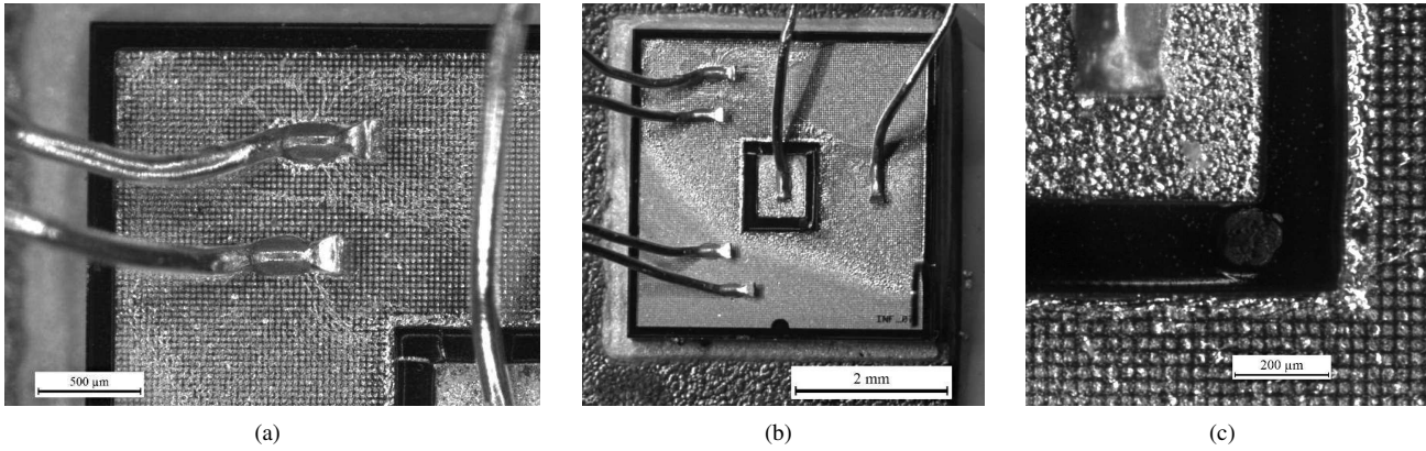
Fig. 10. Photographs of the SiC JFET #2 after destructive runaway. The aluminium metallization melted in places, especially around the top left wirebonds (a). This indicates that the surface temperature of the die exceeded 660 °C. Other consequences of the runaway include the lift-off of the polyimide passivation (b), bottom right corner of the die, and a (hardly visible) round mark under the polyimide layer between gate and source (c). The gate is the small aluminium rectangle in the center of the die (b). Note that 5 wirebonds are connected to the source, 4 to supply the current, the last one to measure the voltage (Kelvin configuration).
