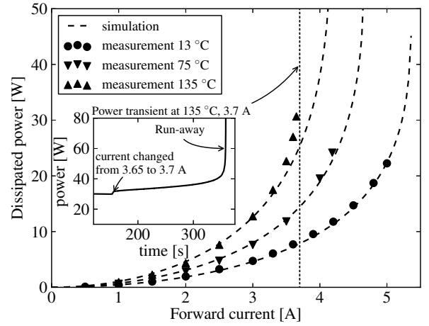
Fig. 7. Power dissipated by JFET #1 (4.5 K/W thermal resistance) as a function of its forward current, and for 3 different ambient temperatures (13, 75, and 135 °C). The symbols correspond to measurements, the lines to simulation (computing the solutions of (8)). The device entered (non-destructive) thermal runaway at 3.7 A, 135 °C ambient temperature. The transient power measured during runaway is plotted in the detail graph.
