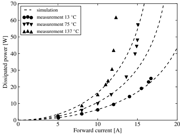
Fig. 9. Power dissipated by JFET #3 (2 K/W). For the “13 °C” curve, the power was limited by the cooling capability of our test bench. In all cases, the dissipated power was limited to 110 W to avoid the destruction of the device.
