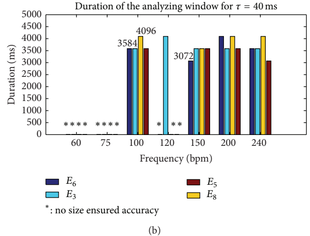
FIGURE 5: Duration of the analyzing window W required to reach an error of at least 0.25 bpm with the autocorrelation estimator ( I_2 ) and with a SNR > 0.6 dB.
