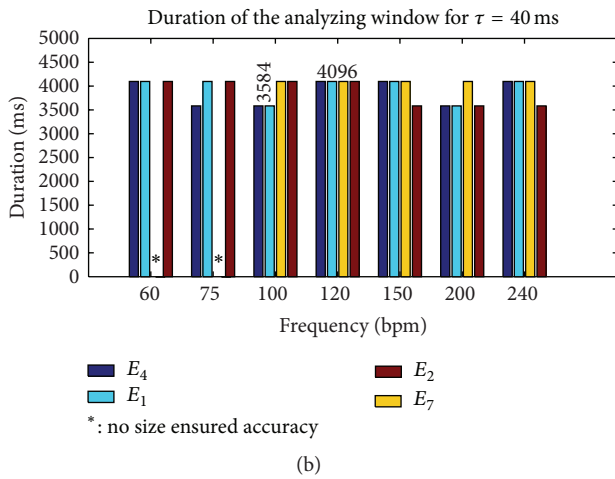
FIGURE 4: Duration of the analyzing window W required to reach an error of at least 0.25 bpm with the autocorrelation estimator ( I_1 ) and a SNR > 0.6 dB.
