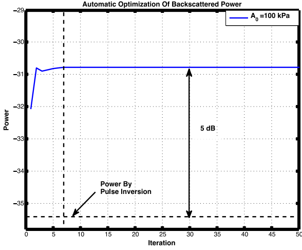
Fig. 3 Automatic optimization of the backscattered power of chirp y(t) with initial driving pressure 100 kPa.
