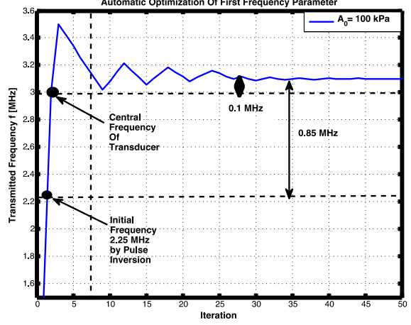
Fig. 4 Automatic optimization of the first chirp parameter f for initial driving pressure 100 kPa.
