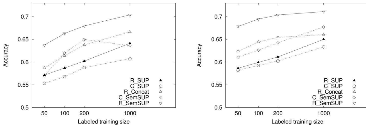
Figure 2: Accuracy of different strategies with respect to four different labeled training size and when the percentage of positive class is below (left) and above (right) 15%, on the NUS-WIDE-LITE dataset. Performance are averaged over 22 classes and 50 random splits.
