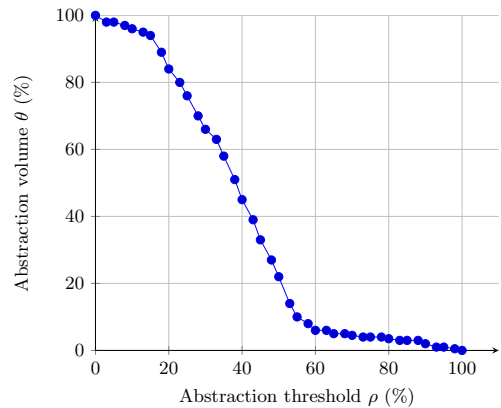
Figure 7: Abstraction Volume
