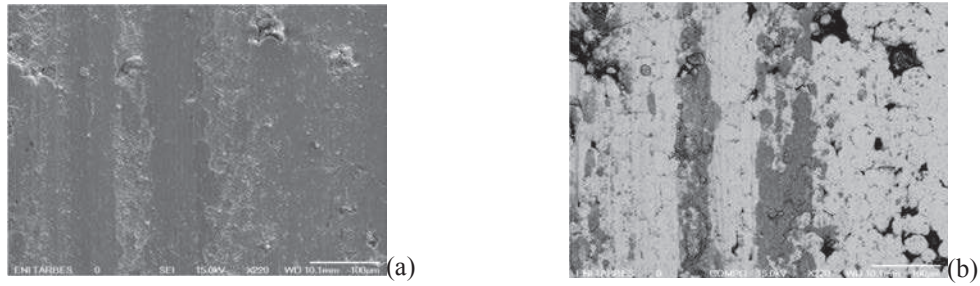
Figure 17: Observations by SEM of the St10BN with two different magnification observation modes: secondary electron and backscattered electron with chemical contrast.
