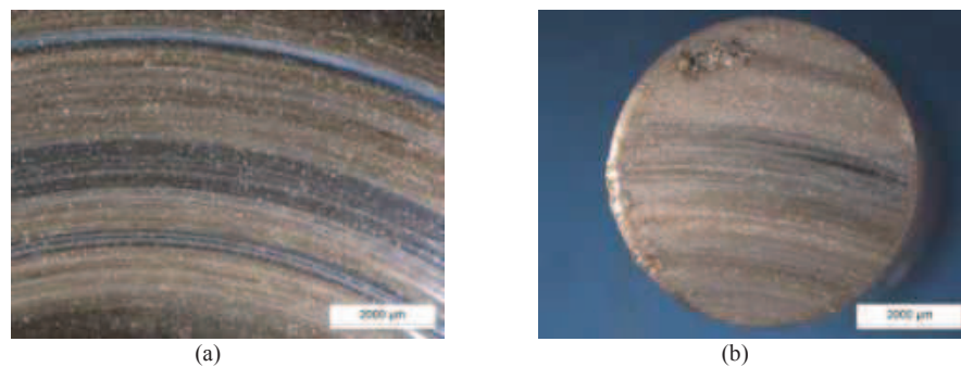
Figure 7: Binocular microscopy images (a) of the Stellite sample (b) and of the pin.
