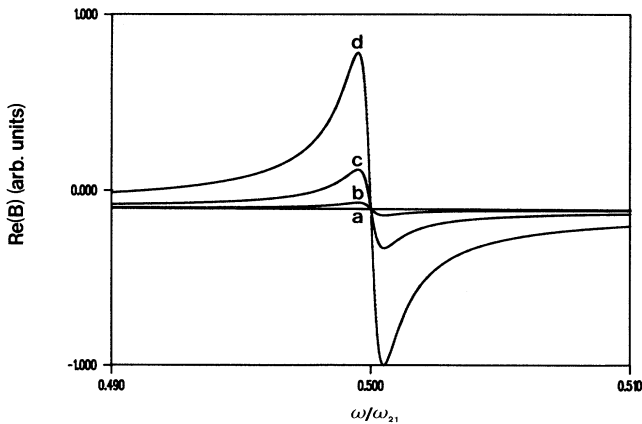
FIG. 3. Real part of the two-photon degenerate four-wave-mixing nonlinear response. The values of the parameters are \mu_{ab}=1 , \Gamma_2=10^3 , \Gamma_1=1 , D=0 , \omega_{21}=10^6 , and (a) d=0 , (b) d=2 , (c) d=5 , and (d) d=10 .
