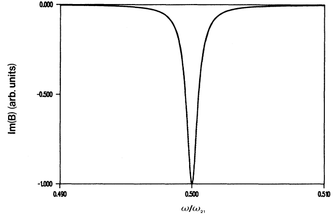
FIG. 6. Influence of the rotational diffusion on the imaginary part of the two-photon degenerate four-wave-mixing nonlinear response. The values of the parameters are \mu_{ab}=1 , \Gamma_2=10^3 , \Gamma_1=1 , d=5 , and \omega_{21}=10^6 . No dependence with respect to D is observed.
