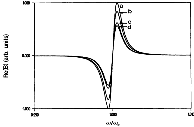
FIG. 7. Influence of the rotational diffusion on the real part of the one-photon degenerate four-wave-mixing nonlinear response. The values of the parameters are \mu_{ab}=1 , \Gamma_2=10^3 , \Gamma_1=1 , d=5 , \omega_{21}=10^6 , and (a) D=0 , (b) D=0.1 , (c) D=1 , and (d) D=10 .
