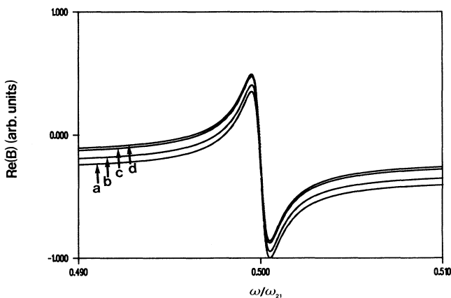
FIG. 5. Influence of the rotational diffusion on the real part of the two-photon degenerate four-wave-mixing nonlinear response. The values of the parameters are \mu_{ab}=1 , \Gamma_2=10^3 , \Gamma_1=1 , d=5 , \omega_{21}=10^6 , and (a) D=0 , (b) D=0.1 , (c) D=1 , and (d) D=10 .
