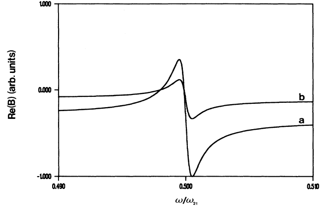
FIG. 9. Influence of the field polarization on the real part of the two-photon degenerate four-wave-mixing nonlinear response. The values of the parameters are \mu_{ab}=1 , \Gamma_2=10^3 , \Gamma_1=1 , d=5 , \omega_{21}=10^6 , and D=0 : (a) parallel polarizations; (b) perpendicular polarizations.
