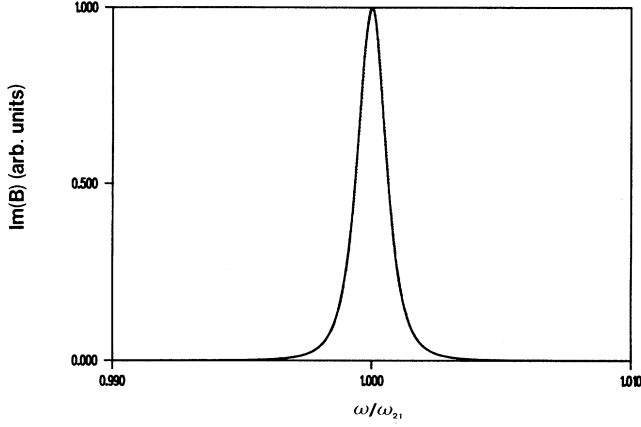
FIG. 2. Imaginary part of the one-photon degenerate four-wave-mixing nonlinear response. The value of the parameters are \mu_{ab}=1 , \Gamma_2=10^3 , \Gamma_1=1 , D=0 , and \omega_{21}=10^6 . No variations are observed as d varies.
