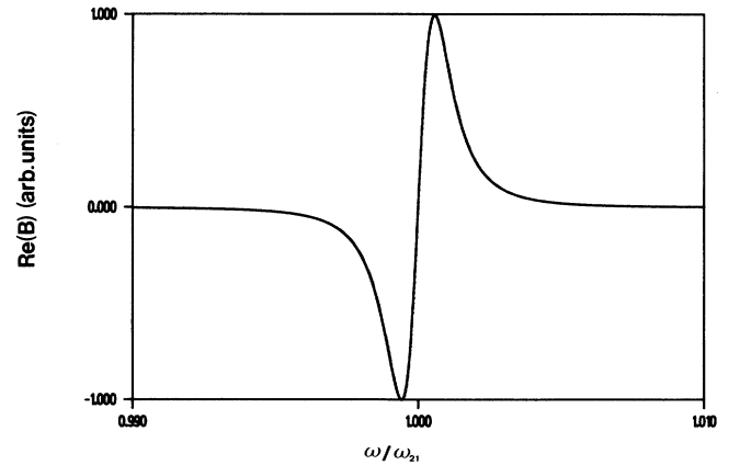
FIG. 1. Real part of the one-photon degenerate four-wave-mixing nonlinear response. The values of the parameters are \mu_{ab}=1 , \Gamma_2=10^3 , \Gamma_1=1 , D=0 , and \omega_{21}=10^6 . No variations are observed as d varies.
