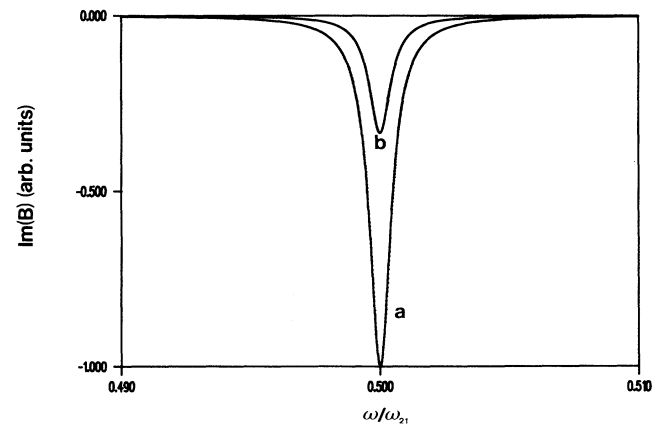
FIG. 10. Influence of the field polarization on the imaginary part of the two-photon degenerate four-wave-mixing nonlinear response. The values of the parameters are \mu_{ab}=1 , \Gamma_2=10^3 , \Gamma_1=1 , d=5 , \omega_{21}=10^6 , and D=0 : (a) parallel polarizations; (b) perpendicular polarizations.
