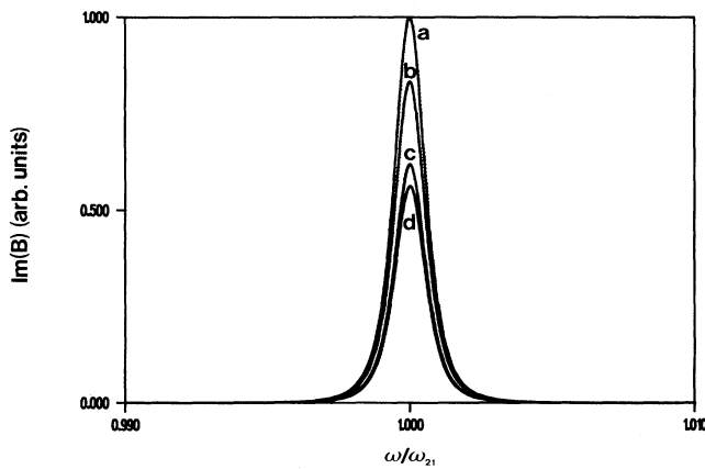
FIG. 8. Influence of the rotational diffusion on the imaginary part of the one-photon degenerate four-wave-mixing nonlinear response. The values of the parameters are \mu_{ab}=1 , \Gamma_2=10^3 , \Gamma_1=1 , d=5 , \omega_{21}=10^6 , and (a) D=0 , (b) D=0.1 , (c) D=1 , and (d) D=10 .
