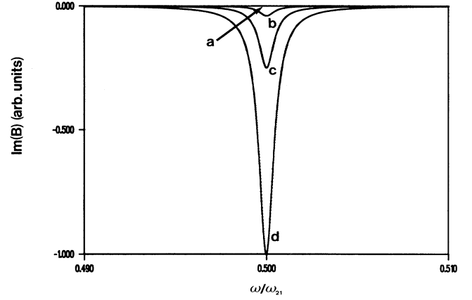
FIG. 4. Imaginary part of the two-photon degenerate four-wave-mixing nonlinear response. The values of the parameters are \mu_{ab}=1 , \Gamma_2=10^3 , \Gamma_1=1 , D=0 , \omega_{21}=10^6 , and (a) d=0 , (b) d=2 , (c) d=5 , and (d) d=10 .
