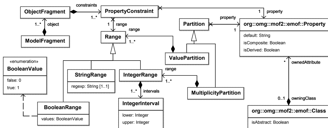
Figure 5 – Meta-model for test criteria definition
