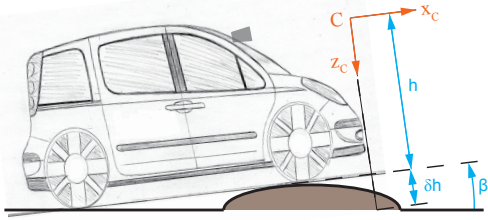
Fig. 2. Parameter variation while climbing a speed bumper
