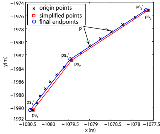
Fig. 3. Illustration of the 2 stages lane marking fitting. The tolerance is 20 centimeters.
