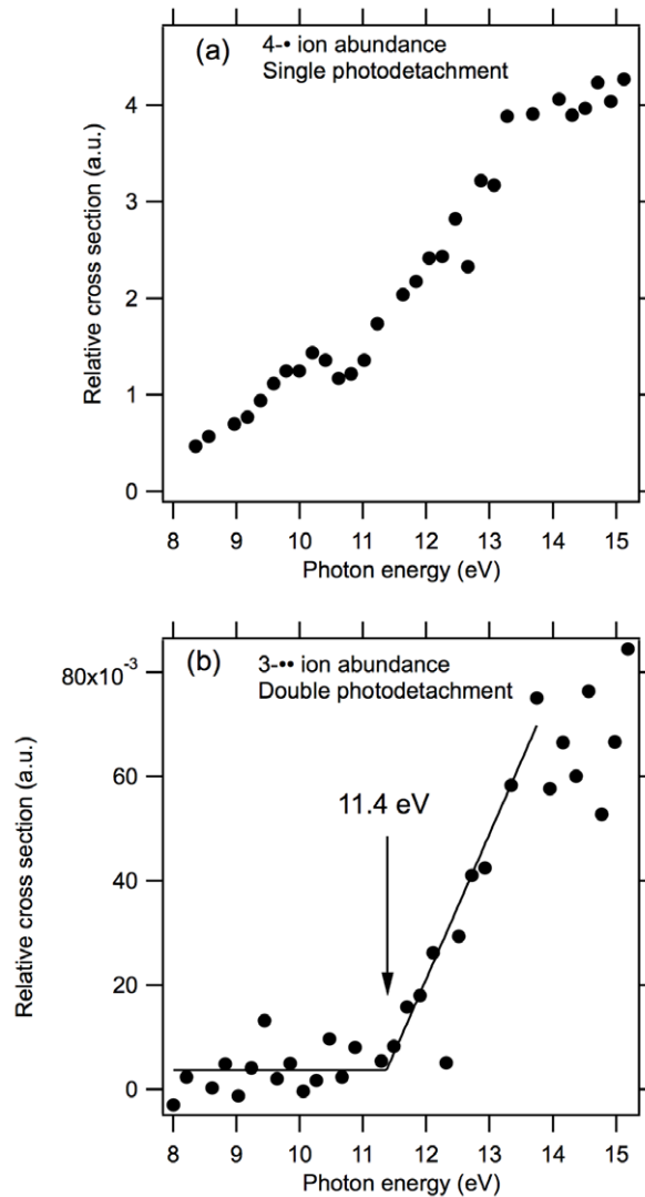
Figure 2. Partial relative cross section (see text) in the 8–15.2 eV range for 90 ms irradiation duration for (a) single photodetachment and (b) double photodetachment. The solid line is a Wannier-type linear fit to the data (see text).
