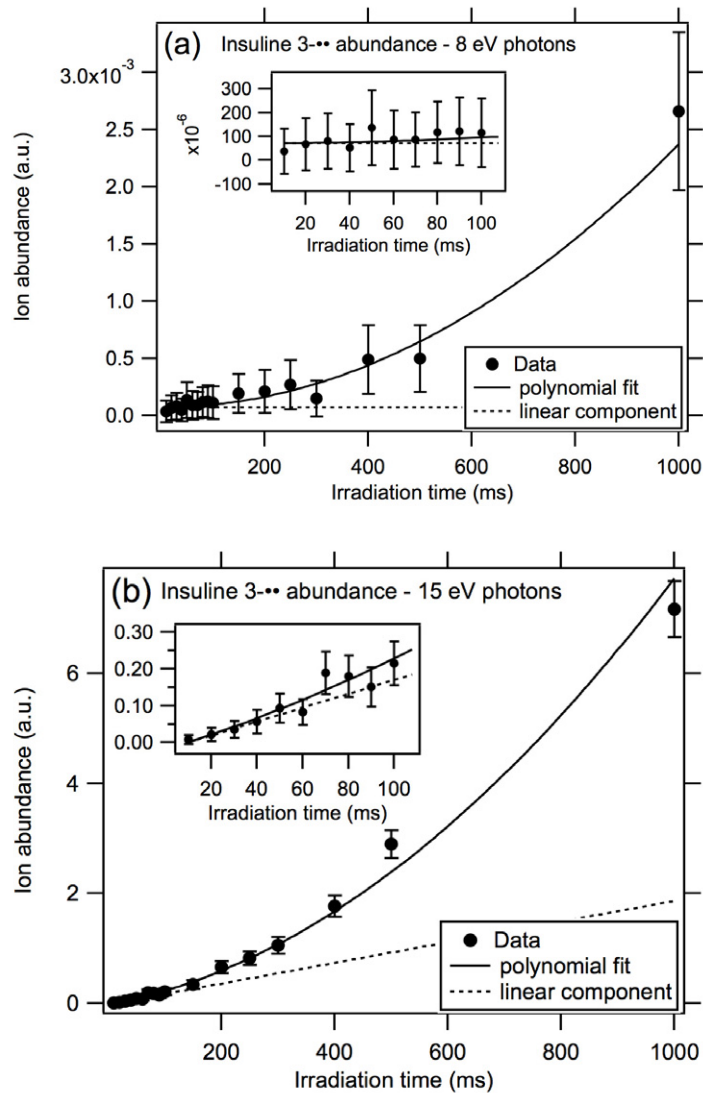
Figure 3. Ion abundances for the double photodetachment product ion [M - 5H]^{3-} at (a) 8 and (b) 15 eV recorded as a function of the irradiation time in the 10–1000 ms range. The data were least square fitted by a second-order polynomial: a + bt + ct^2 , where a , b and c are fitting coefficients and t stands for time in ms. The dotted lines labeled on the graph as a linear component represent the linear components of the fit expressed by a' + b't .
