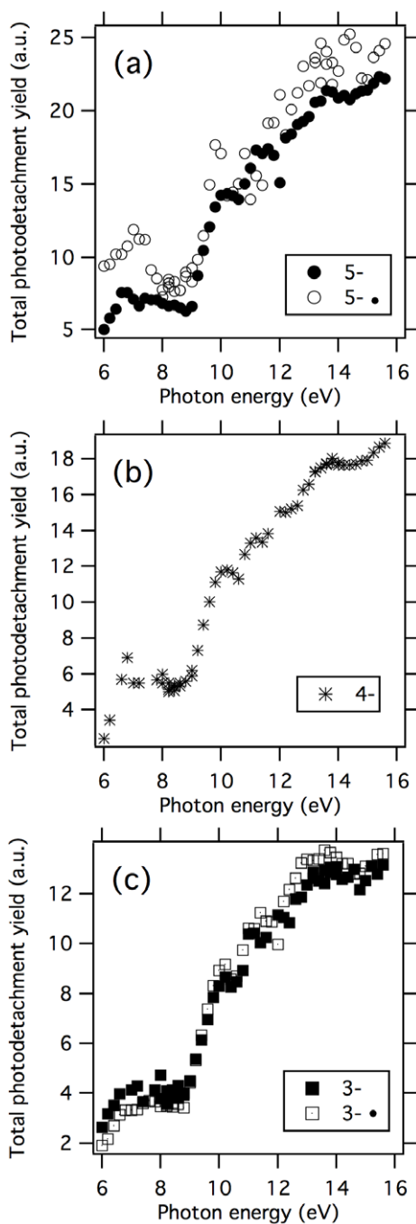
Figure 4. Total photodetachment yields as a function of the photon energy as calculated by -\ln(\text{precursor}/(\text{precursor} + \text{products}))/\varphi , where \varphi is the photon flux, ‘precursor’ is the intensity of the parent peak and ‘products’ represents the total intensity of the peaks corresponding to the oxidized species (i.e. protein that has lost electrons). Yields are compared for closed-shell precursors with 3-, 4- and 5-charge states and for open-shell precursors labelled 3 – • and 5 – •.
