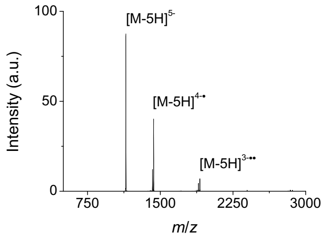
Figure 1. Mass spectrum after irradiation with 15 eV photons and 400 ms irradiation duration of the insulin [M - 5H]^{5-} anion.
