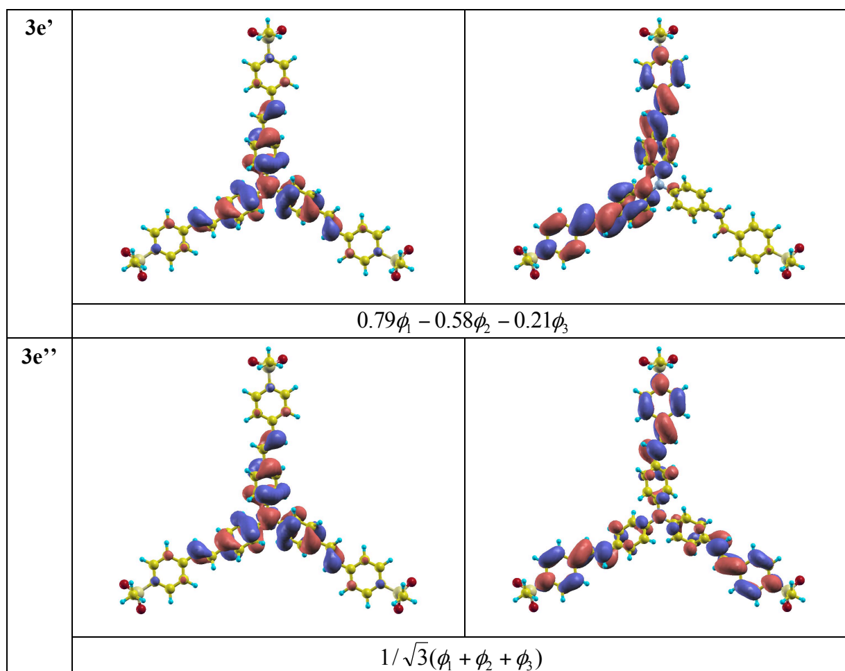
Figure 7. Natural transition orbitals of chromophores 1-3 (absorption). State labeling is given on Scheme 2. 78,79
