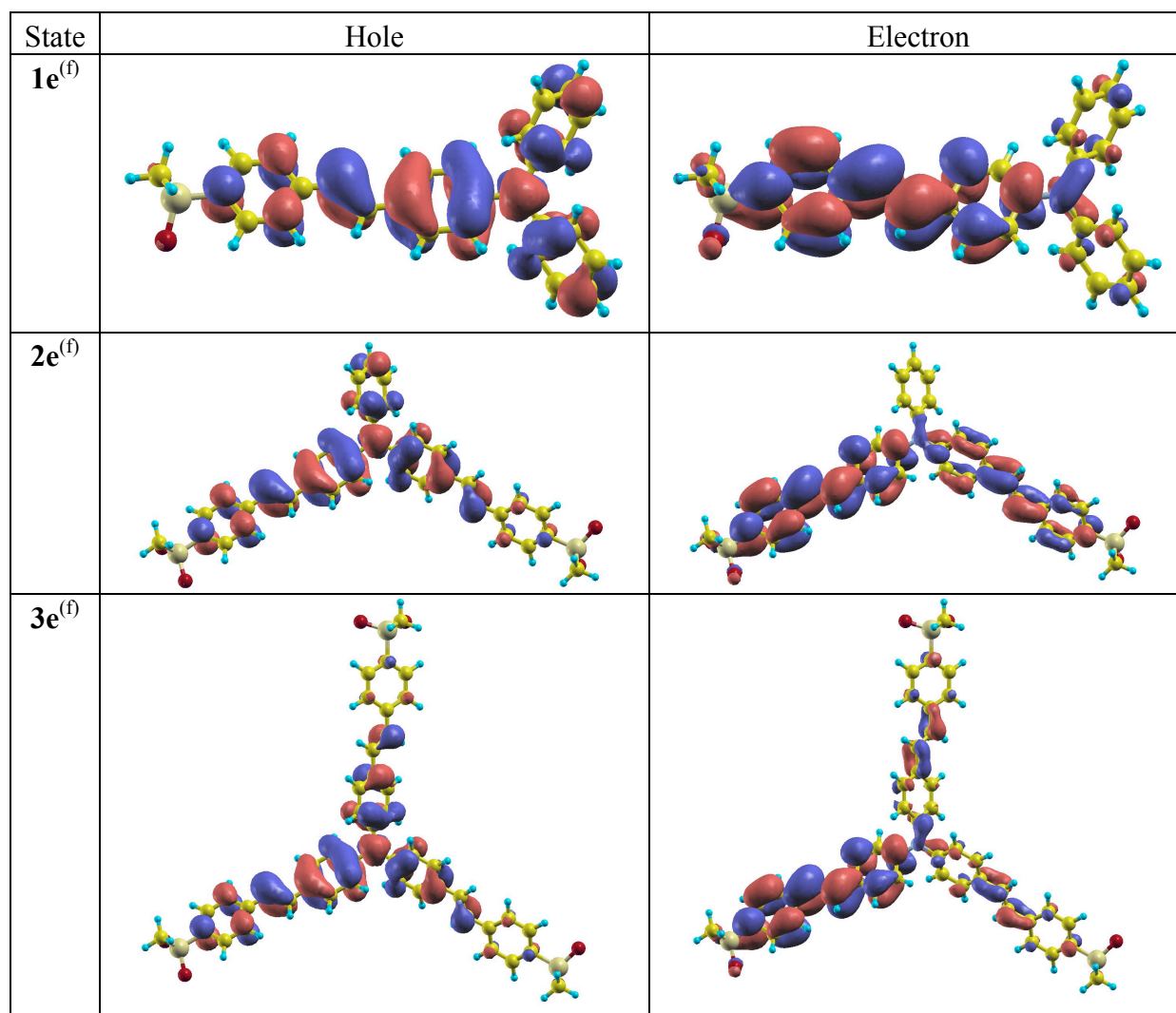
Figure 8. Natural transition orbitals of chromophores 1-3 (emission). 78,79
