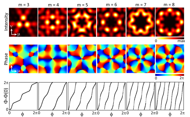
FIG. 10 (color online). Far-field characteristics for m = 3, 4, 5, 6, 7, and 8 . First and second rows: Fraunhofer diffraction intensity and phase patterns in the reciprocal coordinate system, here displayed in the range -0.1 \leq (\mu, \nu) \leq 0.1 . Third row: Azimuthal dependence of the phase along the circle that passes by the intensity maxima. Simulation parameters: \sigma = -1 , w/R = 0.02 , \lambda = 500 \text{ nm} , and R = 10 \mu\text{m} .
