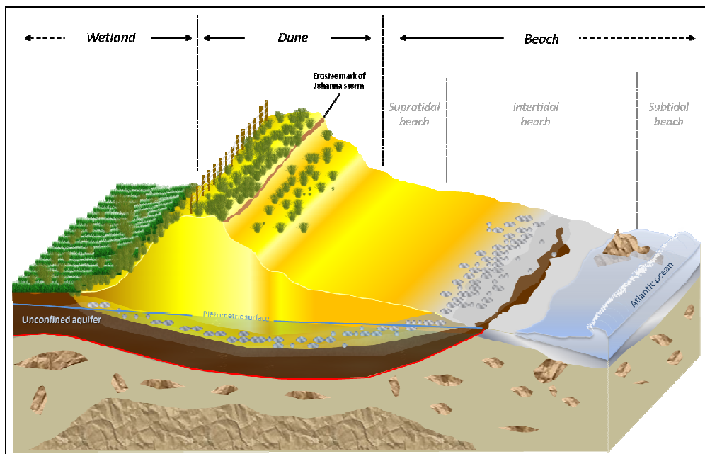
Figure 2. Hypothetic geological scheme of Vougot area.
