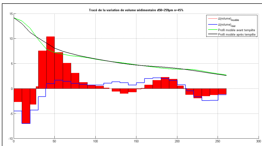
Figure 9: Volume variation of sediments during Johanna storm along modeling profile
