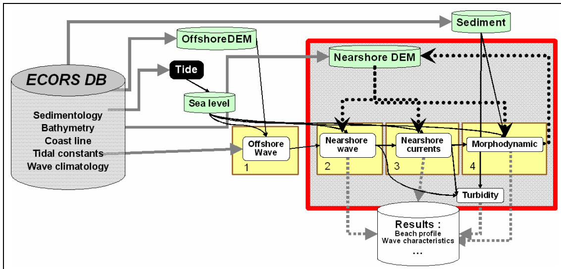
Figure 6. The conceptual model of ECORS simulator second level (from Garlan et al., 2011).
