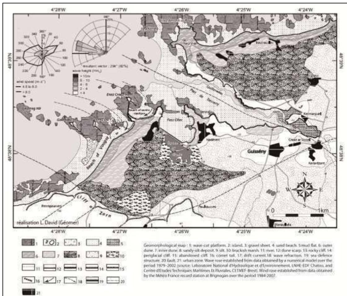
Figure 3. Geomorphological map of coastal area of Guissény town, centralize on Vougot beach (from Suanes et al. 2011)
