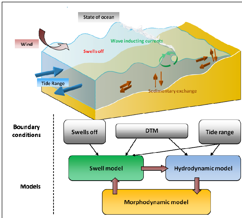
Figure 5. Conceptual scheme of ECORS modeling strategy (from Garlan et al., 2011, modified)
