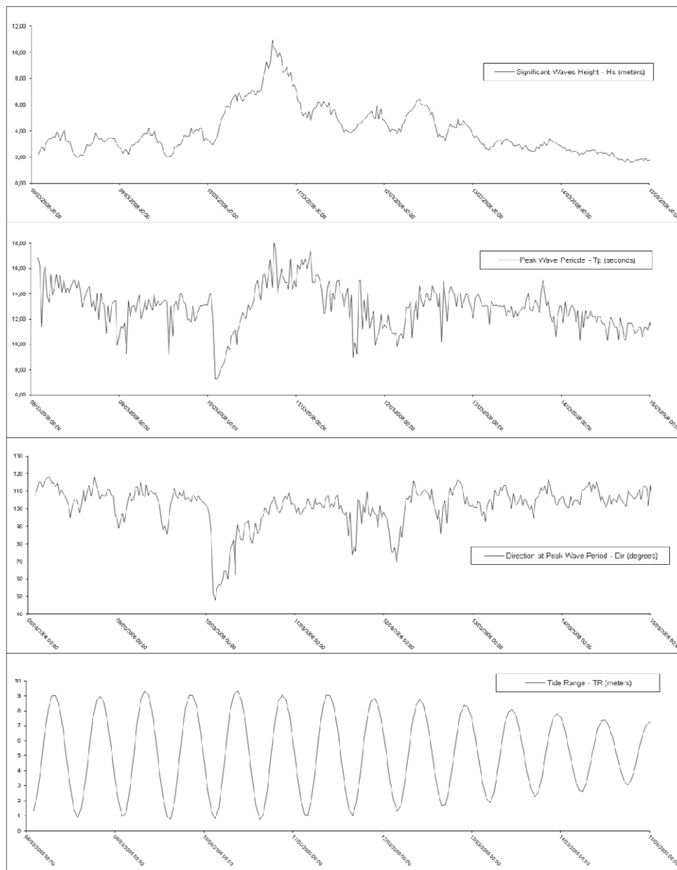
Figure 4. Hydrodynamical data during Johanna storm and apply to SWAN-XBeach models
