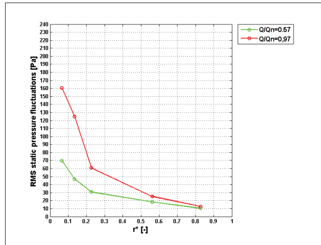
Figure 6: RMS Pressure
