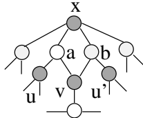
Figure 9: Vertex x is a degree 4 vertex that is a mirror of the degree three vertex v .
