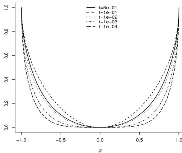
FIGURE 3. D_t(\rho) for various values of the threshold t along with the correlation \rho
