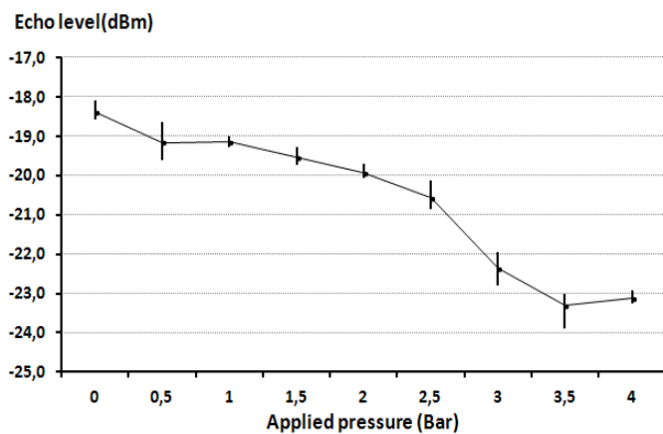
Fig. 1: Measured echo level of passive EM pressure sensor versus applied pressure at the beat frequency f_{ant} of the antenna scattering mode.
