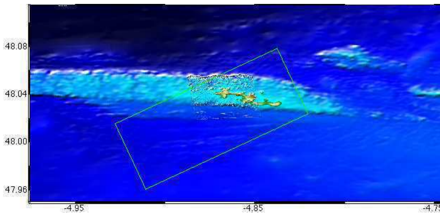
Figure 4: Bathymetry of Sein surroundings. The green tilted rectangle shows the BOSZ grid extension.
