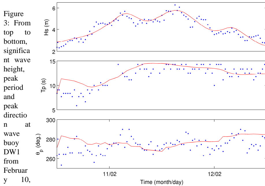
Figure 3: From top to bottom, significant wave height, peak period and peak direction at wave buoy DW1 from February 10, 12h to February 12, 12h. Blue dots, observations, red line WW3 model results.
