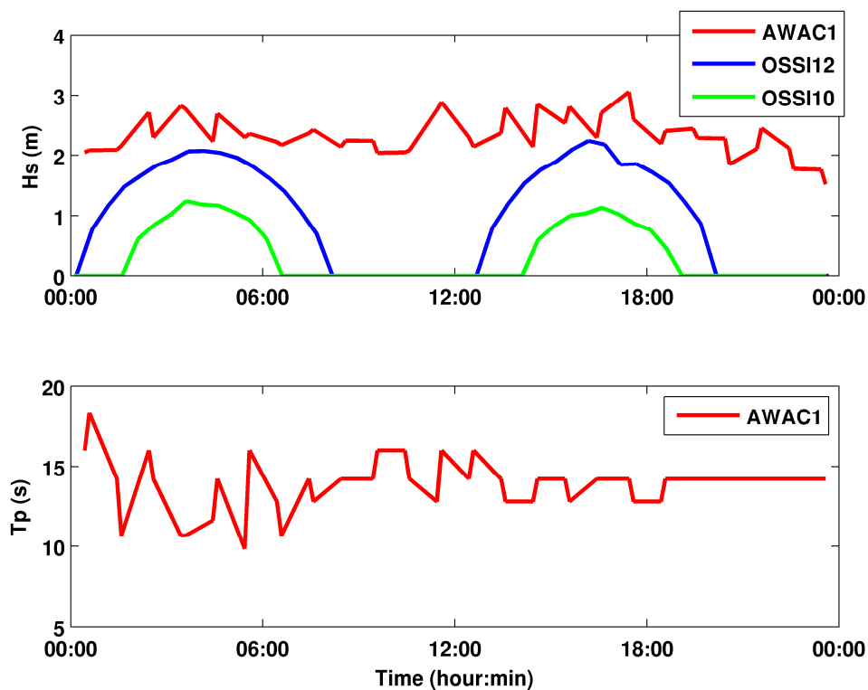
Figure 5: Significant wave height measured at AWAC1, OSSI12 and OSSI1 and peak period at AWAC1 on February 11, 2013.
