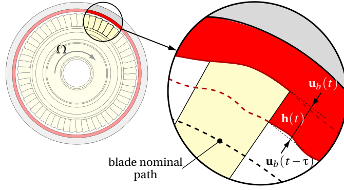
Figure 4: Schematic of abrasion material removal
