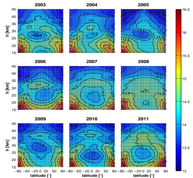
Fig. 7. Latitude–altitude maps of OCIO slant column densities (log scale, \text{cm}^{-2} ) retrieved from GOMOS measurements for years 2003–2011. Latitude range of 80^\circ S– 80^\circ N, altitude range of 15–45 km.
