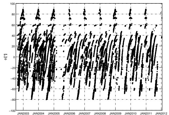
Fig. 2. Latitudinal distribution of the GOMOS transmittance measurements used to retrieve OCIO as a function of time.
