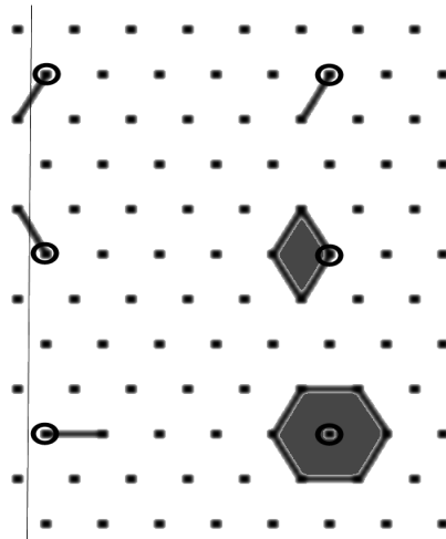
Figure 2: Edge effects when computing an hexagonal dilation with three successive dilations by segments: on the left, points generated by dilations in directions 1 and 3 fall outside the image window and do not contribute to the next dilations.
