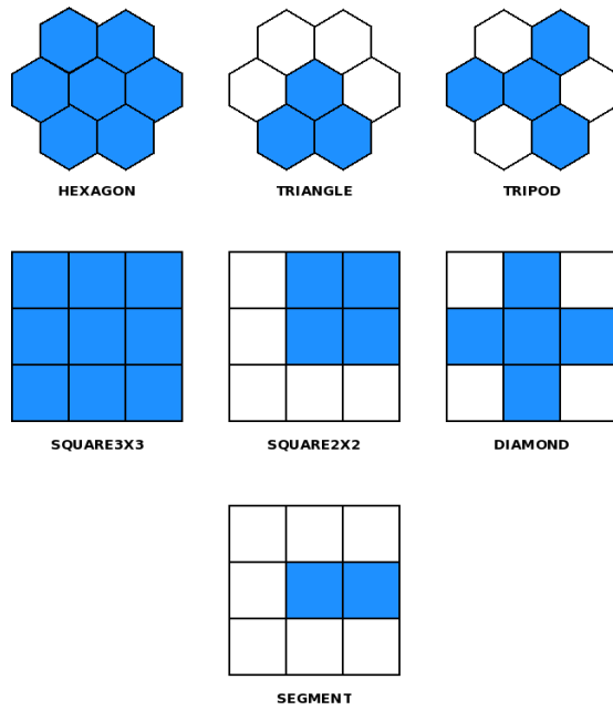
Figure 3: Some structuring elements present in the Mamba library.
