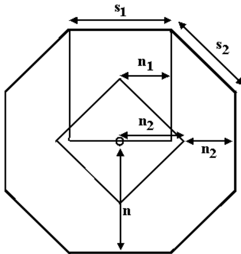
Figure 4: size of the octagon compared to the respective sizes of the square and of the diamond used to get it.
