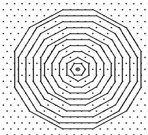
Figure 7: Successive dodecagons generated by the above procedure.
