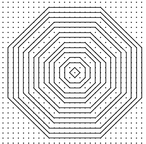
Figure 5: Successive octagons generated by the above algorithm.
