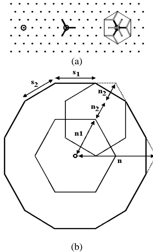
Figure 6: (a) generation of a conjugate hexagon of size 1 by two successive tripods. Note the size of the conjugate hexagon compared to its embedding hexagon. (b) Relations between the size of the dodecagon and the sizes of the hexagon and conjugate hexagon.
