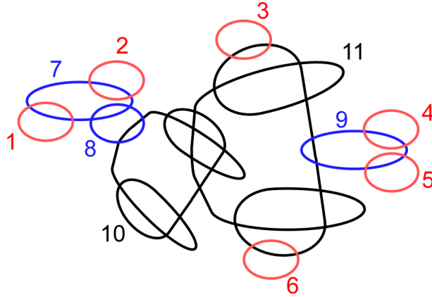
Figure 13: An 11-tuple of nonoriented curves.
