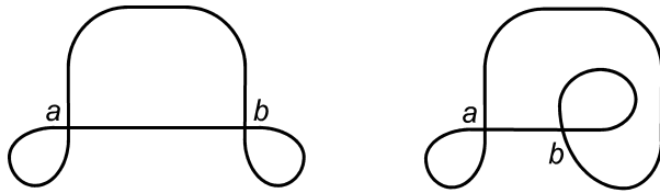
Figure 1: Curves with Gauss word aabb .
