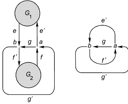
Figure 11: Assertion (1) of Proposition 29
