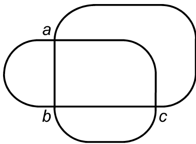
Figure 2: Curve with Gauss word abcabc
