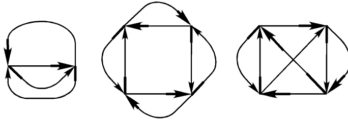
Figure 10: Three atomic t -maps.
