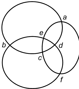
Figure 3: Three intersecting circles
