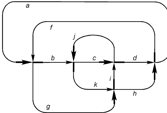
Figure 5: A planar t -map.
