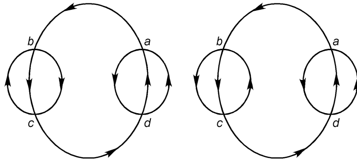
Figure 4: Two nonhomeomorphic embeddings of a same t -map.
