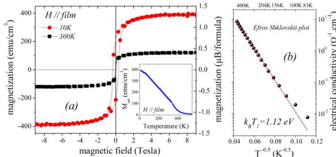
FIG. 3 (a) (color online). Magnetic field dependence of magnetization at 10 K and 300 K for the \text{Fe}_{1.35}\text{Ti}_{0.65}\text{O}_{3-\delta} films, inset: temperature dependence of the saturation magnetization. (Magnetic field along the film plane), (b) Temperature dependence of the DC-electrical conductivity (black dots) fitted with an Efros-Shklovskii (ES) fit at T > 100\text{K} (red line), the upper x-axis is the temperature (in K).
