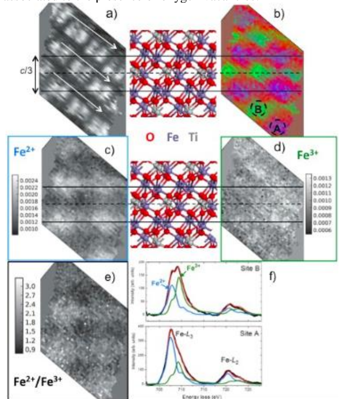
FIG. 1 (color online). (a) STEM HAADF map of the region of interest; (b) reconstructed map combining the O-K, Ti- L_{2,3} , and Fe- L_{2,3} edges (red, green, and blue), (c), (d) and (e) reconstructed maps of the Fe^{2+} , Fe^{3+} spectral weights and the Fe^{2+}/Fe^{3+} ratio, respectively; (f) examples of linear combinations (red line) between Fe^{2+} (siderite – blue line) and Fe^{3+} (hematite – green line) ELNES reference spectra fitting experimental ones (black line) acquired on an Fe-rich (site A) or a mixed Fe/Ti (B) site (each single spectrum was acquired in 100 ms). White arrows in Fig 1 (a) indicate the scan direction. Fe, Ti, and O atoms of the structural model (inner upper schemes) are illustrated in violet, gray, and red respectively.
