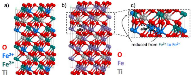
FIG. 2 (color online). (a) Fe oxidation state distributions in \text{Fe}_{1.5}\text{Ti}_{0.5}\text{O}_3 (Ti atoms are all \text{Ti}^{4+} ), (b) \text{Fe}_{1.5}\text{Ti}_{0.5}\text{O}_{3-\delta} model including a single oxygen vacancy, (c) Distribution of Fe oxidation states in the two layers around the oxygen vacancy site. In all figures, Ti atoms are labelled in grey and O in red. In Fig. (b) Fe atoms are in violet while in Figs. (a) and (c) \text{Fe}^{2+} and \text{Fe}^{3+} are in blue and green, respectively.
