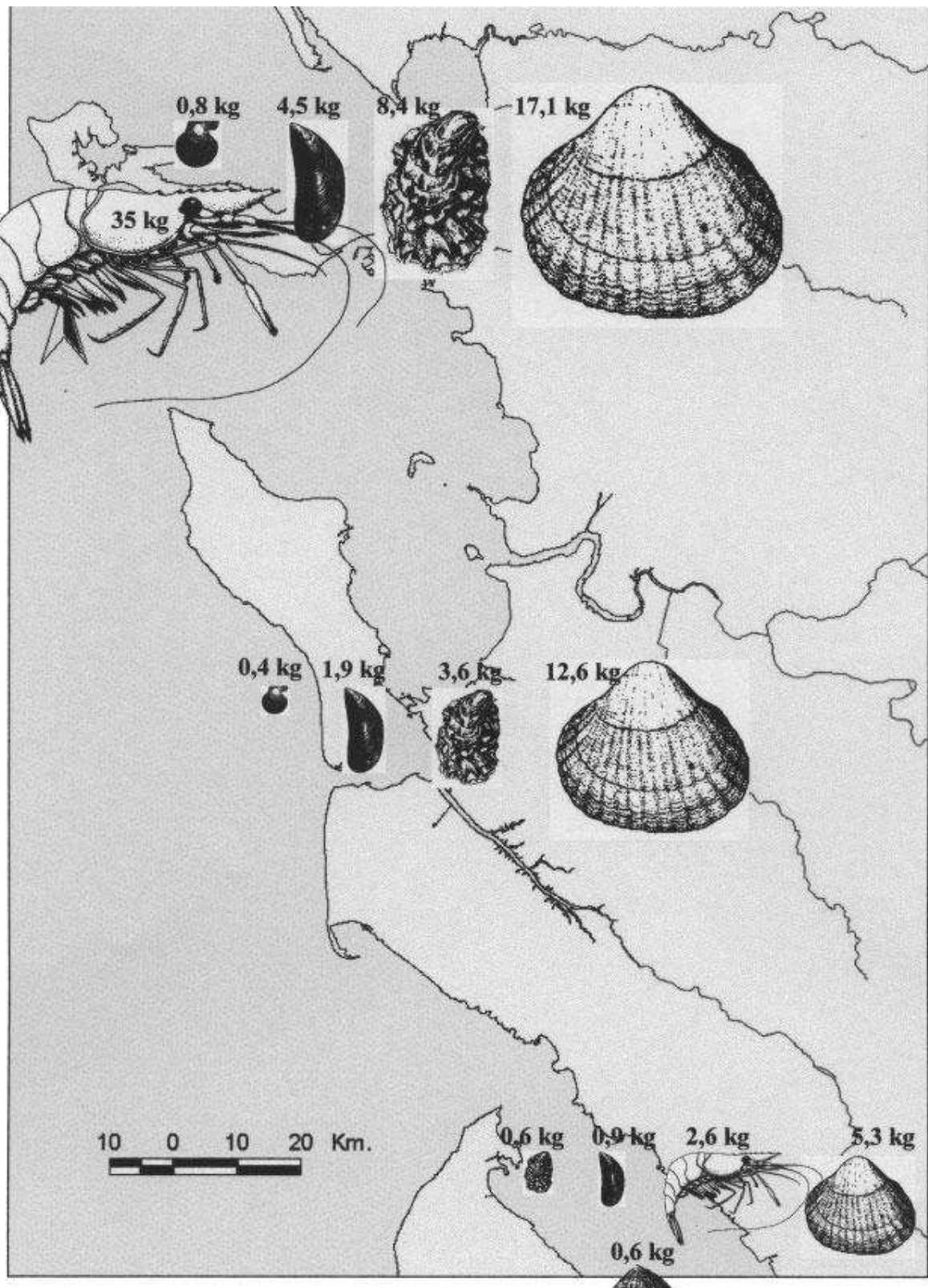
FIGURE 4. — Weekly shellfish consumption in a 65 Kg man sufficient to reach the Cd Provisional Tolerable Weekly Intake (PTWI): 7 \mu\text{g}\cdot\text{Kg}^{-1} . Calcul includes a Cd input due to normal food and drink which represents 38 % of the PTWI.
