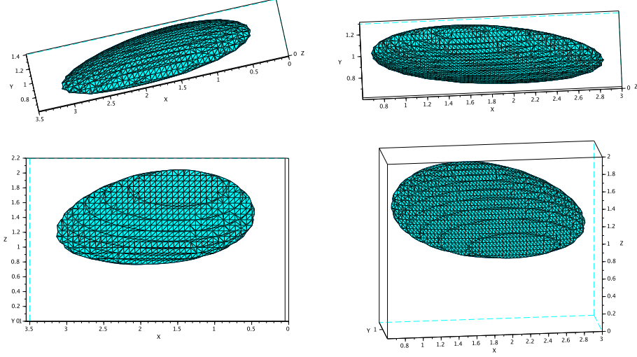
FIGURE 10. Domains \Delta(\lambda, \mu, \nu) > 4.95 and \Delta(\lambda, \mu, \nu) > 5 , with x = \coth(\lambda - \mu) - \frac{1}{\lambda - \mu} , y = \lambda , and z = \nu .
