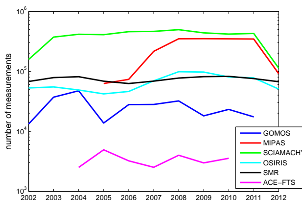
Figure 1. Number of measurements in each year and for each instrument. Number of MIPAS and SCIAMACHY measurements decrease significantly in 2012 due to the loss of Envisat. GOMOS data from year 2012 are not included in HARMOZ, because GOMOS experienced instrumental problems at that time.
