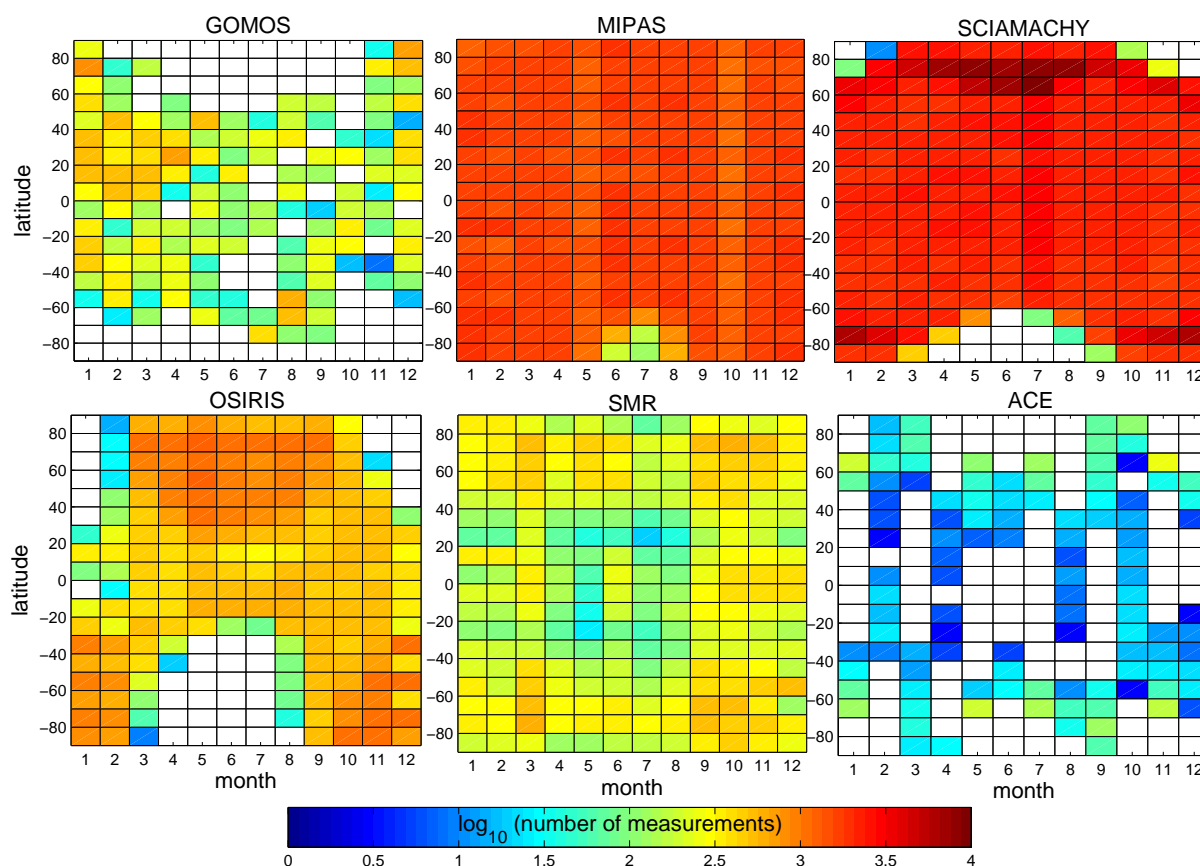
Figure 2. Logarithm of number of measurements in 10^\circ latitude zones and in each month of year 2008.
