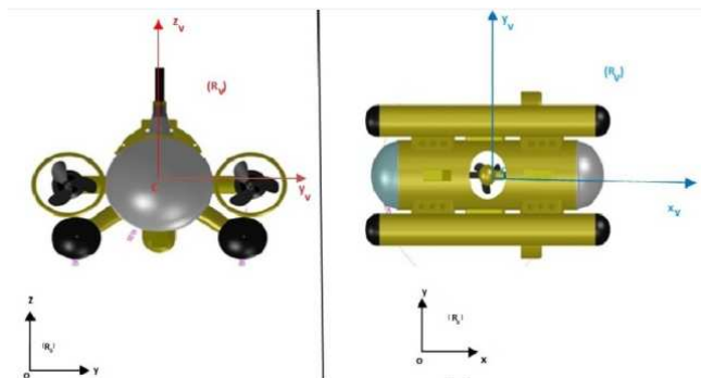
Figure 2: The global and local references frames attached to the ROV.
