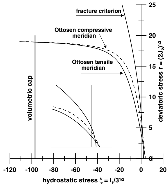
Fig. 13. Yield criteria on the meridian plane.
