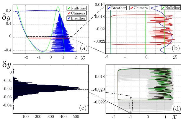
FIG. 4: (Color on line) Nullcline numerical analysis of the chimera, \beta = 0.6 , x_0 = 1 . (a): Chaotic breathers (blue), as in Fig.3(c,d), and chimera (red) along the nullcline (green). (b): Zoom-in of (a) close to y = 0 . (c): Histogram for \delta y -values at the condition x = -1.0 (see circle in (d)), over 10,000 delays. (d): Chimera wandering in the (x, \delta y) -plane, for two (black and green) and 100 (light gray) successive delays.
