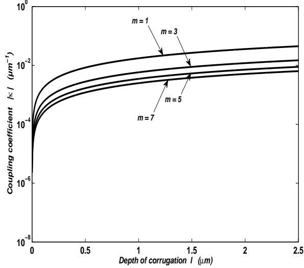
Figure 2: Coupling coefficient \kappa versus the corrugation depth l for different values of Bragg's order m . (simulation data: n_1 = 2.2112, n_2 = 2.2174, n_3 = 1, d = 5 \mu\text{m} and r = 0.5 ).
