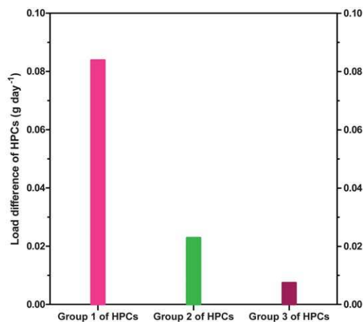
Fig. 4 Load difference for the three groups of HPCs (g d -1 ) between upstream and downstream from Rennes.
