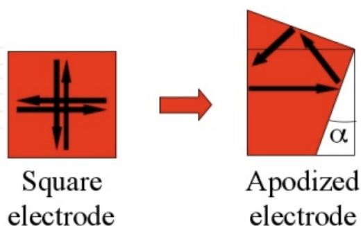
Figure 4. Apodization applied to a square electrode
