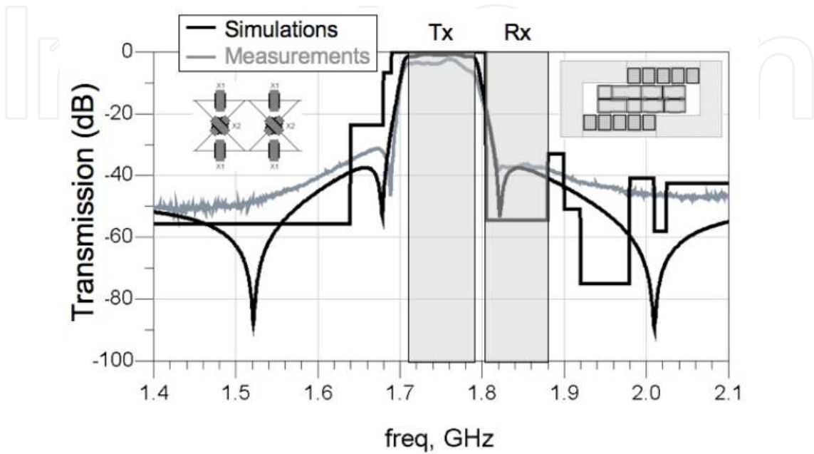
Figure 25. 2-stage lattice filter compared to UMTS standard
