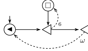
Figure 4. An RLA representing Monday.
