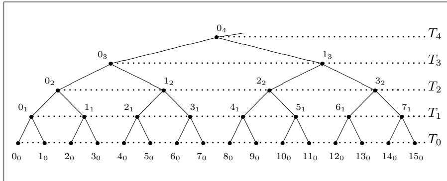
Figure 1. The 2-refinable upward unbounded layered structure
