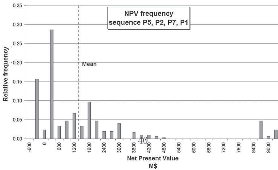
Fig. 14. Frequency and behaviour for non-dominated tricriteria optimization.
