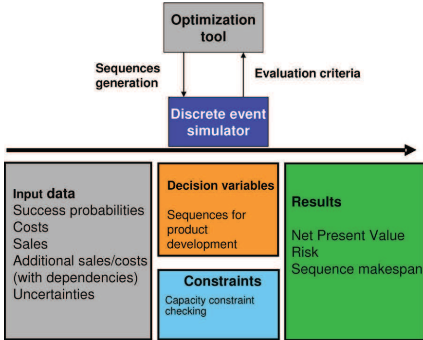
Fig. 4. SED-optimization framework.
