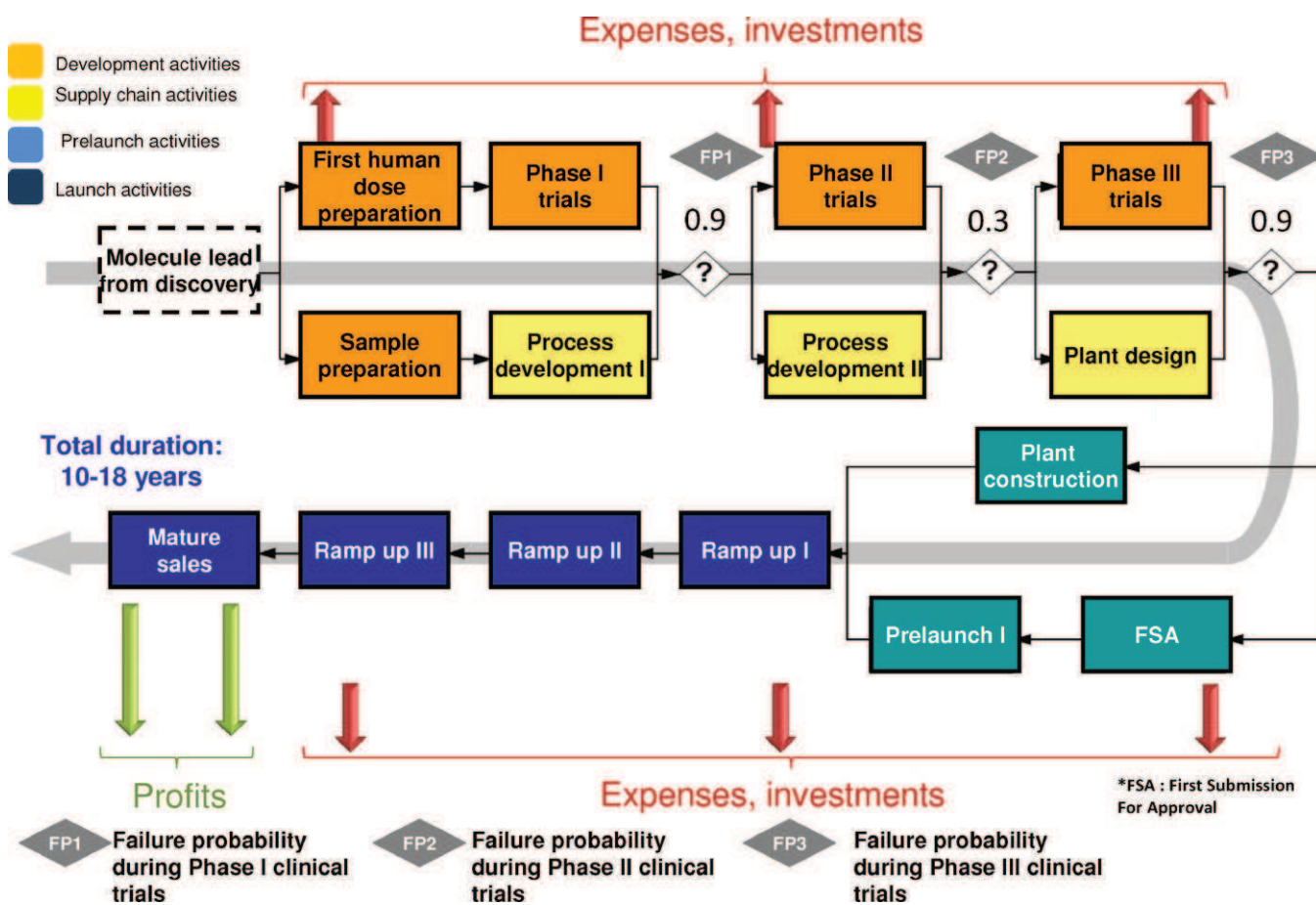
Fig. 1. Process for drug development.
