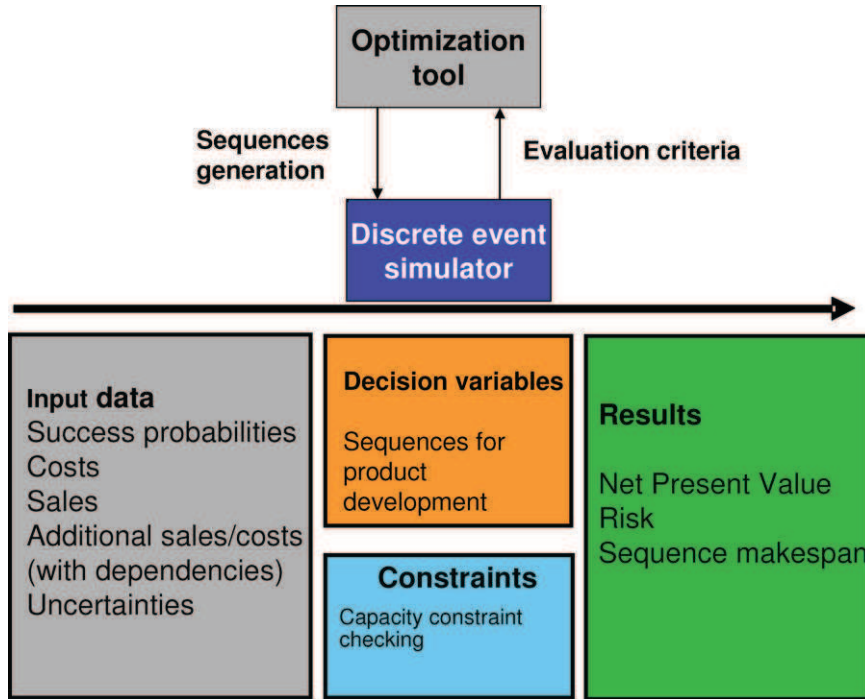
Fig. 4. SED-optimization framework.
