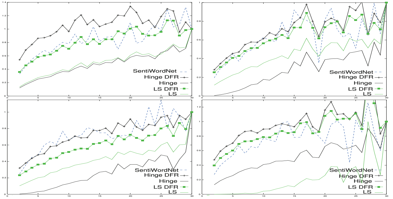
Figure 3: Subjectivities (SentiWordNet & Models) wrt to the word frequencies using bigram description. This curves show a slightly different behaviors from the unigrams (cf Fig. 2). Datasets from top left to bottom right: books, electronics, DVD, kitchen. For each dataset, we consider the weight vector of the best model in term of accuracy (evaluated in cross-validation).
