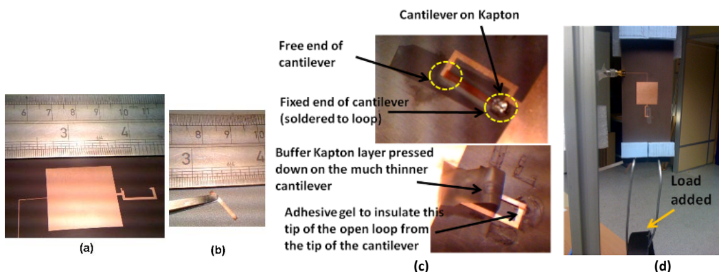
Figure 4 : Fabricated portions of the passive EM strain-sensing device : (a) metallic patch connected to the open loop; (b) cantilever to be connected to one edge of the open loop; (c) the open loop with the cantilever connected at one edge (one end of the cantilever is free, i.e., not connected to the loop) and (d) the assembled high-sensitive strain-sensing device and measurement setup
