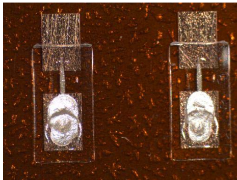
Figure 7 : Two micro-fluidics half-wavelength dipoles of the temperature sensor (length = 3.6mm, width = 1mm and thickness = 1\mu m ) printed on Kapton substrate ( 9 \times 23.4 \times 0.127 mm^3 ). The gap at the center of each dipole is loaded by a micro-channel (cross section 50\mu m \times 50\mu m ) filled with liquid metal. The dimensions of the tank are 1.3mm \times 800\mu m \times 50\mu m .
