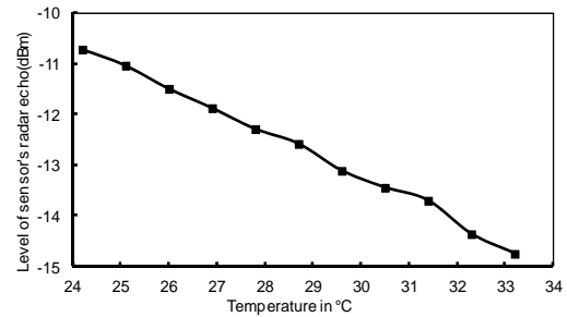
Fig. 7. Measured radar echo level versus temperature.
