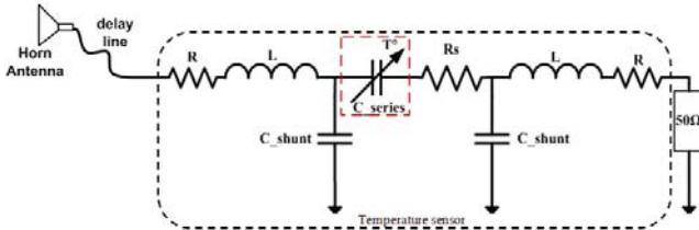
Fig. 4. Equivalent circuit of the micro-system.
