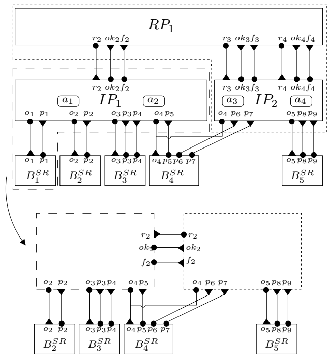
Fig. 14 Merging together components B_1^{SR} and IP_1 , and RP_1 and IP_2 .
