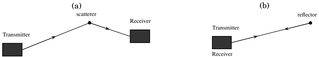
FIGURE 1: (a): Scheme of a Transmit/Receive configuration. (b): Scheme of a Pulse/Echo configuration.
