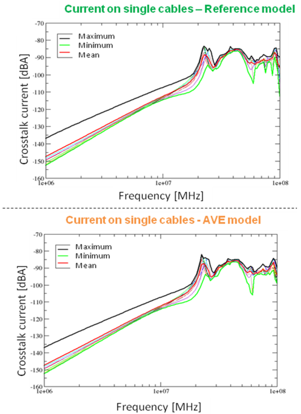
Figure 9. Comparison of crosstalk current on single cables for the 9 coupling from TPC to victim cables between reference model and AVE model
