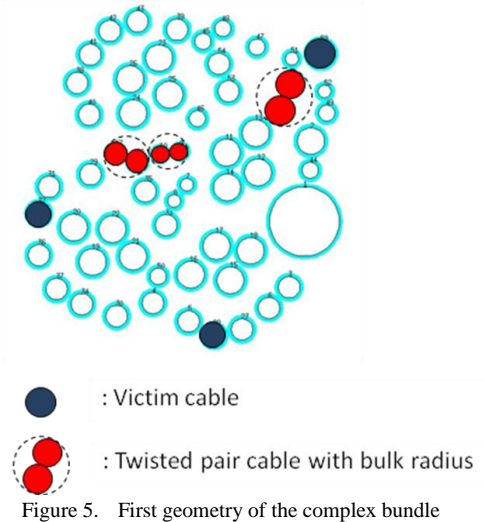
Figure 5. First geometry of the complex bundle
