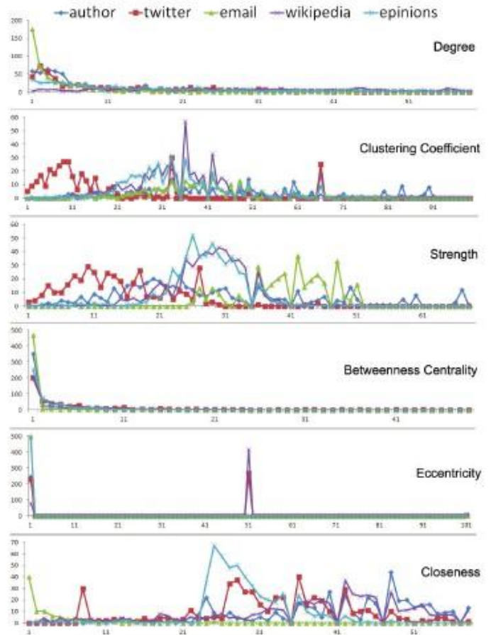
Fig. 2. Calculating different Network Metrics on the Five datasets. Horizontal axis represents bins and vertical axis represents the frequency with which nodes appear in that particular bin.
